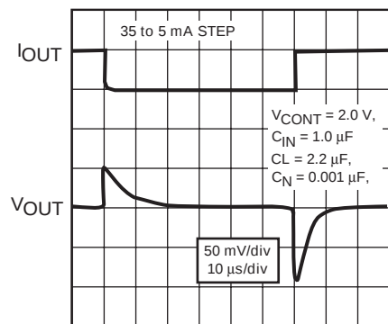
LOAD TRANSIENT 1
