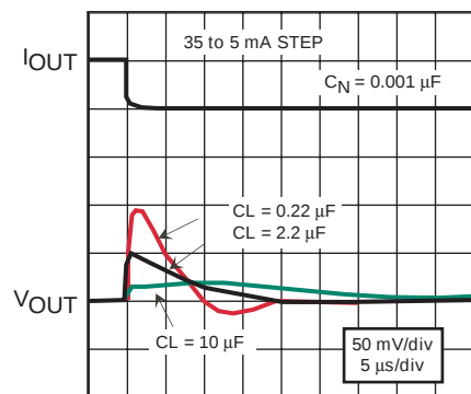
LOAD TRANSIENT 2
