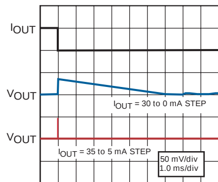
LOAD TRANSIENT 4
