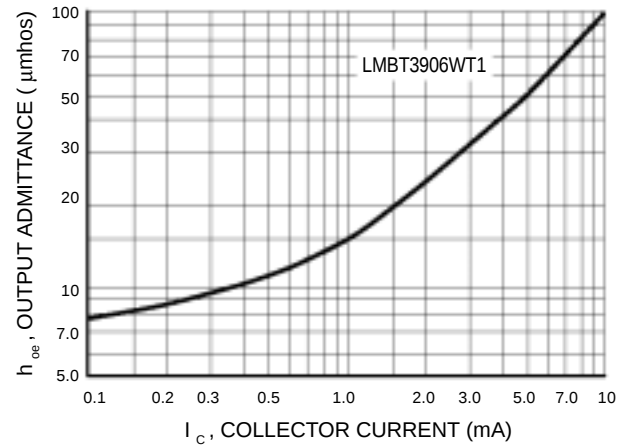
Figure 28. Output Admittance
