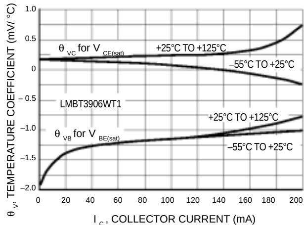
Figure 34. Temperature Coefficients
