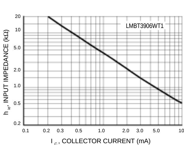
Figure 29. Input Impedance
