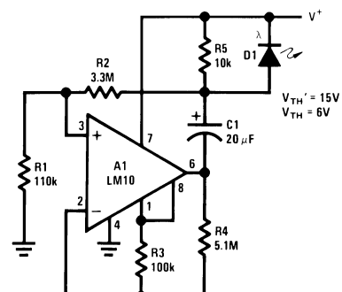
Figure 62. Battery-threshold Indicator
