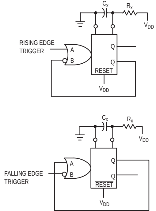
Figure 8. Non-Retriggerable Monostables Circuitry
