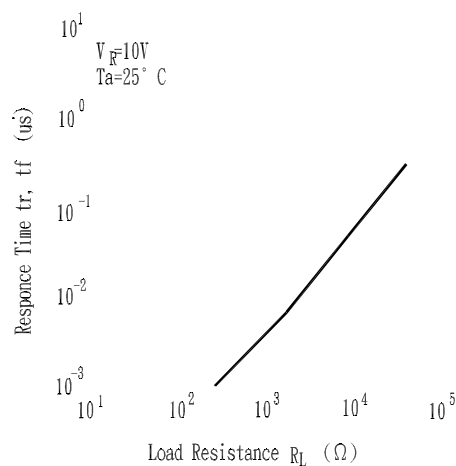
Fig. 6 Response Time vs. Load Resistance
