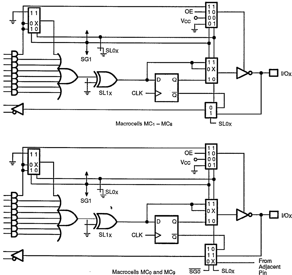
PALCE24V10 Macrocell
