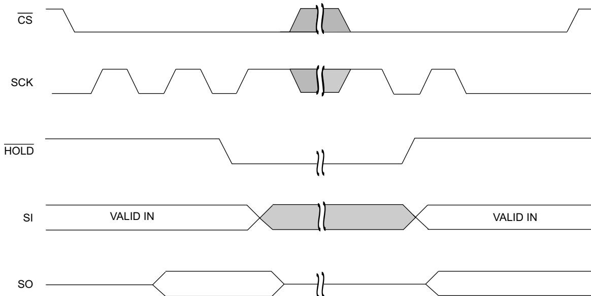
Figure 12. \overline{HOLD} Operation [2]
