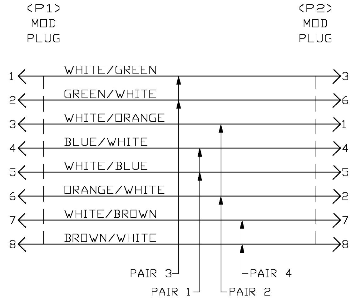
WIRING DIAGRAM CROSSOVER LAN TO 10 BASE T
