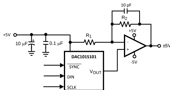
Figure 47. Bipolar Operation
