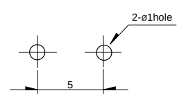
Printed circuit board mounting hole dimensions (When viewed from the switch mounting face)
