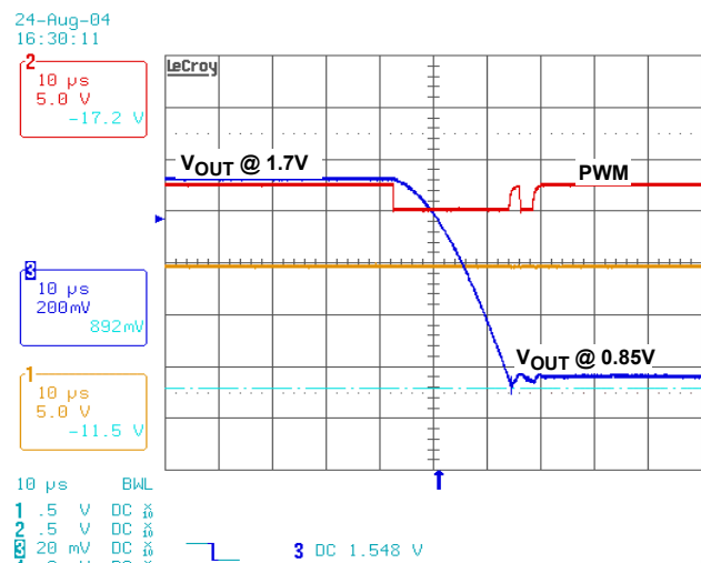
FIGURE 26. 1.7V OVP SHOWING OUTPUT PULLED LOW TO 0.85V AND PWM TRI_STATE
