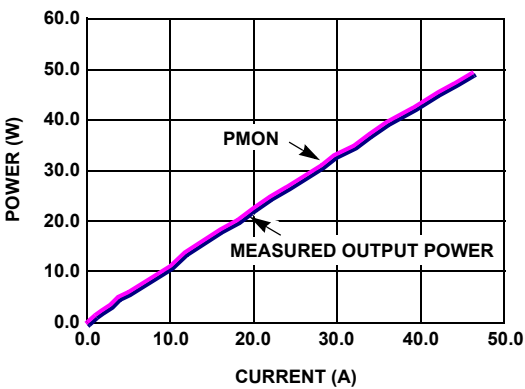
FIGURE 38. POWER MONITOR vs OUTPUT CURRENT
