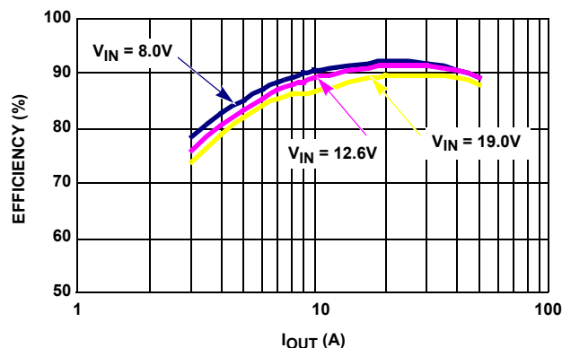
FIGURE 1. ACTIVE MODE EFFICIENCY, 3 PHASE, CCM, PSi# = HIGH, VID = 1.4375V
