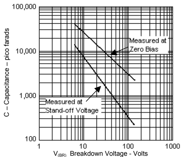
FIGURE 3 Typical Capacitance vs Breakdown Voltage
