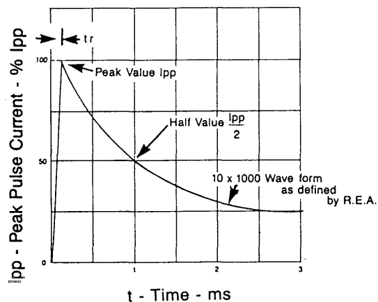
FIGURE 2 Pulse Waveform
