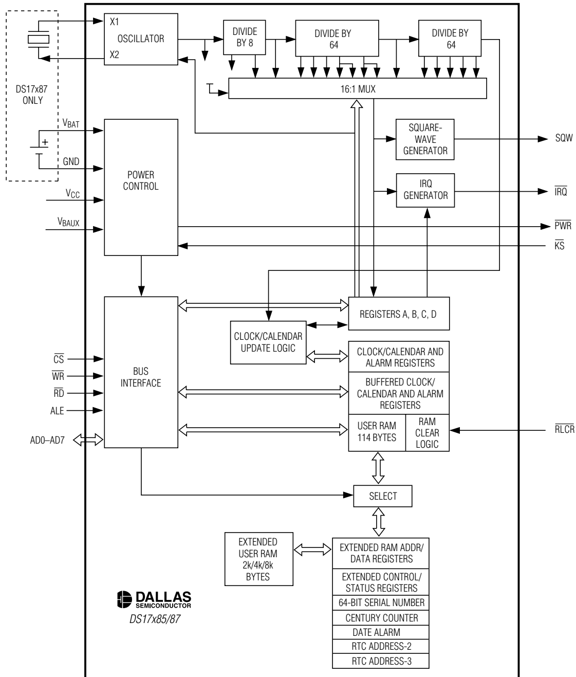
Figure 1. Functional Diagram
