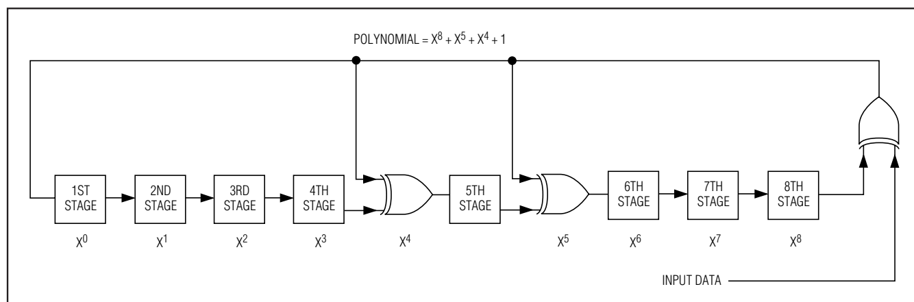
Figure 5. CRC Polynomial
