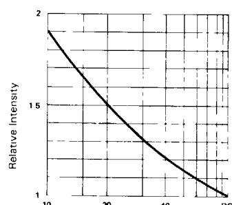
Duty Cycle % Fig 6 LUMINOUS INTENSITY Vs DUTY CYCLE % (AVERAGE I F = 10mA PER SFG)
