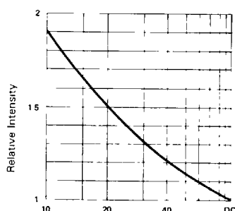
Duty Cycle % Fig 6 LUMINOUS INTENSITY VS DUTY CYCLE % (AVERAGE I = 10\text{mA} PER SEG)
