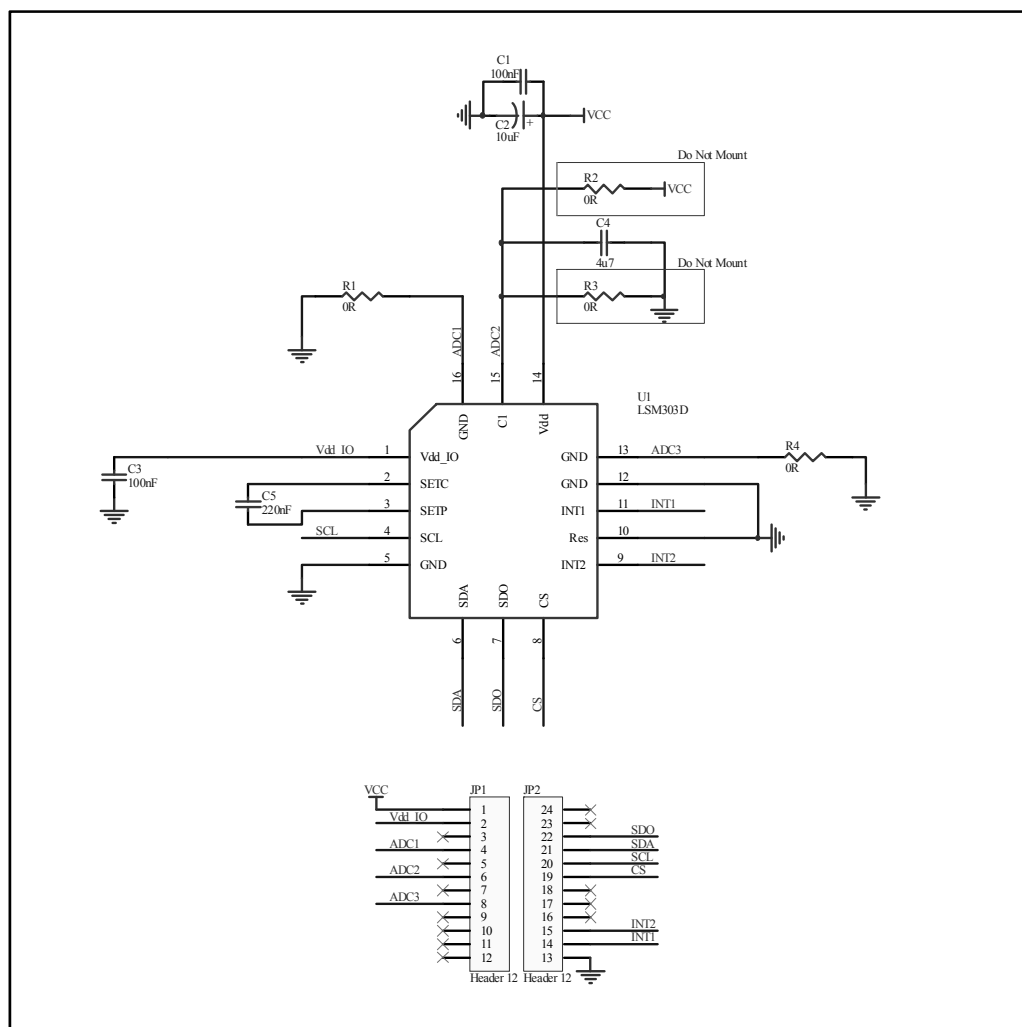
Figure 1: STEVAL-MKI133V1 circuit schematic
