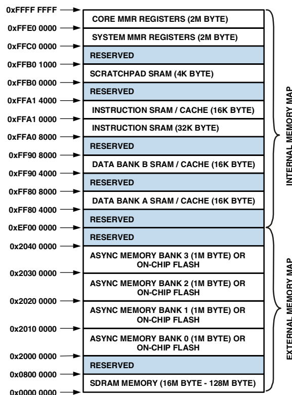
Figure 3. ADSP-BF538/ADSP-BF538F Internal/External Memory Map
