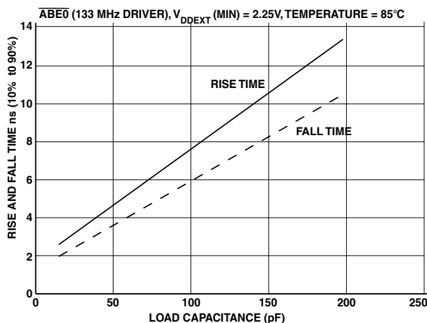
Figure 43. Typical Output Delay or Hold for Driver A at V_{\text{DDEXT}} MIN
