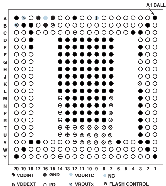
Figure 54. 316-Ball Mini-BGA Pin Configuration (Bottom View)
