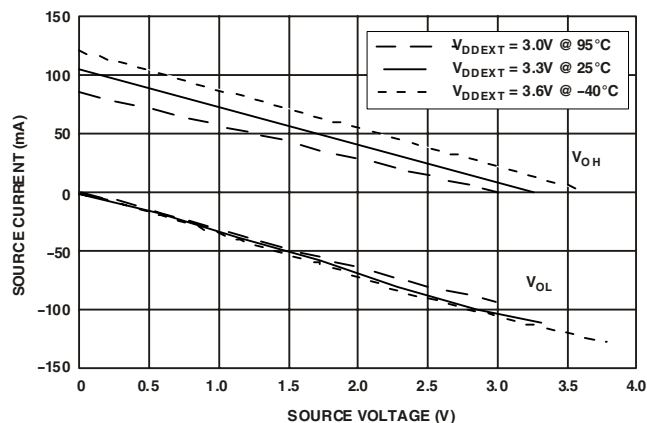
Figure 31. Drive Current A (High V_{DDEXT} )
