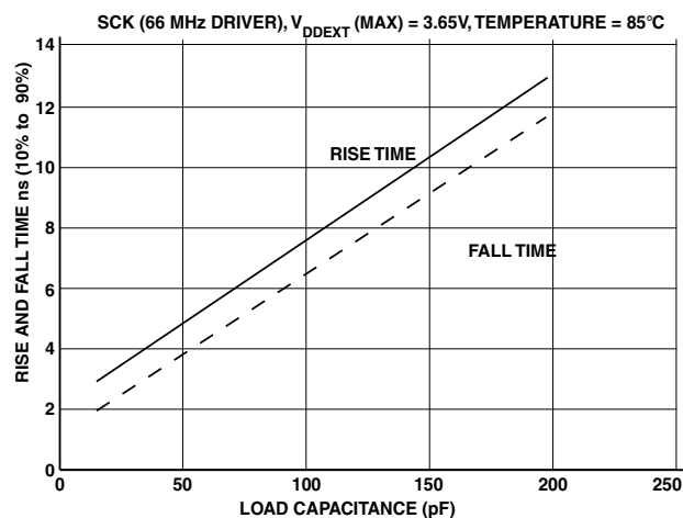
Figure 50. Typical Output Delay or Hold for Driver D at V_{DDEXT} MAX
