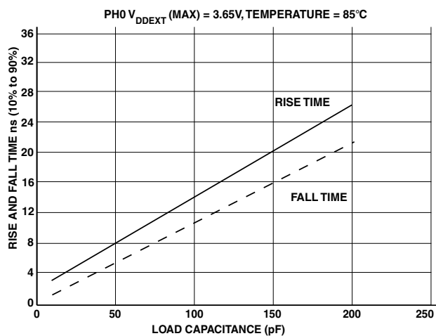
Figure 52. Typical Output Delay or Hold for Driver E at V_{DDEXT} MAX
