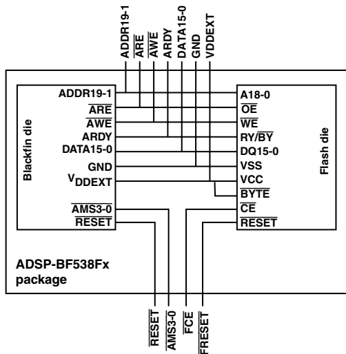
Figure 4. Internal Connection of Flash Memory (ADSP-BF538Fx)
