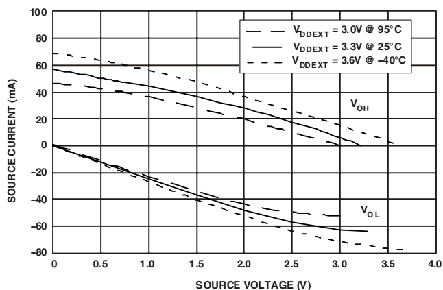
Figure 35. Drive Current C (High V_{DDEXT} )
