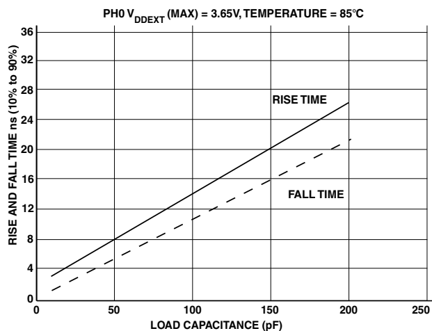
Figure 51. Typical Output Delay or Hold for Driver E at V_{DDEXT} MIN
