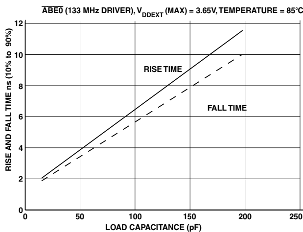
Figure 44. Typical Output Delay or Hold for Driver A at V_{\text{DDEXT}} MAX
