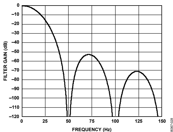
Figure 31. \text{Sinc}^4 Filter Response (FS[9:0] = 96)
