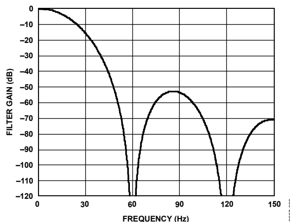
Figure 32. \text{Sinc}^4 Filter Response (FS[9:0] = 80)
