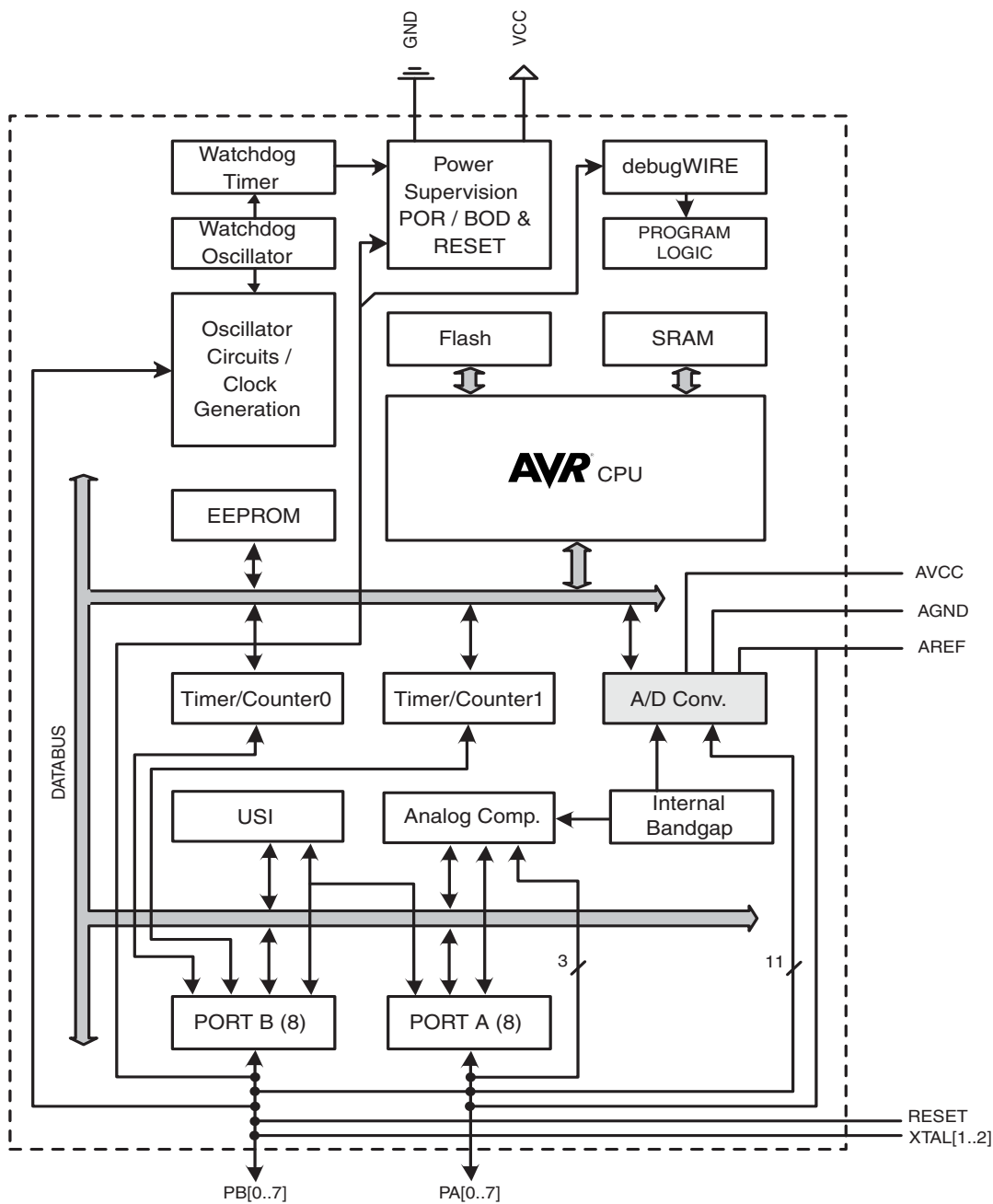
Figure 2-1. Block Diagram
