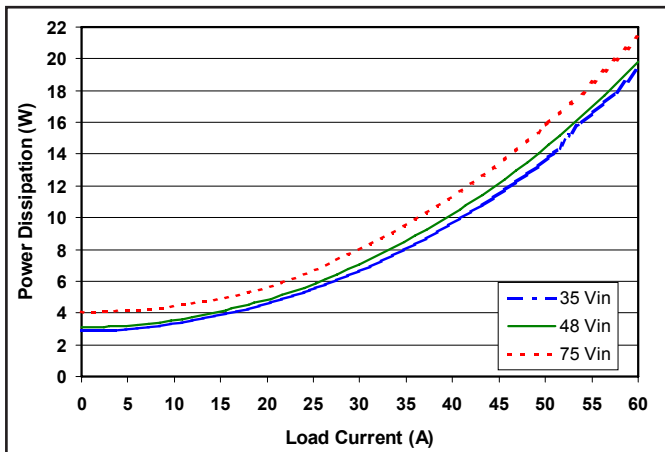
Figure 3: Power dissipation at nominal output voltage vs. load current for minimum, nominal, and maximum input voltage at 25°C (2 output pins).
