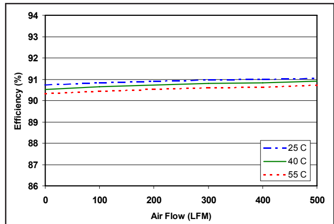
Figure 2: Efficiency at nominal output voltage and 60% rated power vs. airflow rate for ambient air temperatures of 25°C, 40°C, and 55°C (nominal input voltage and 2 output pins).
