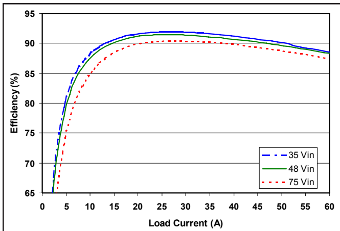
Figure 1: Efficiency at nominal output voltage vs. load current for minimum, nominal, and maximum input voltage at 25°C (2 output pins).
