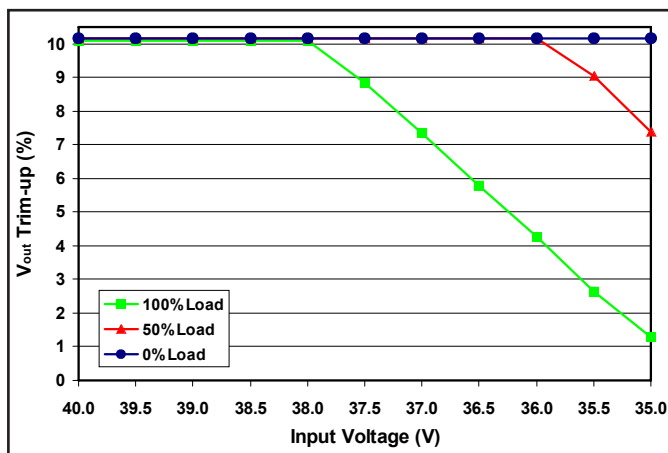
Figure 27: Achievable trim-up percentage vs. input voltage at output loads of 0%, 50% and full load (2 output pin unit).
