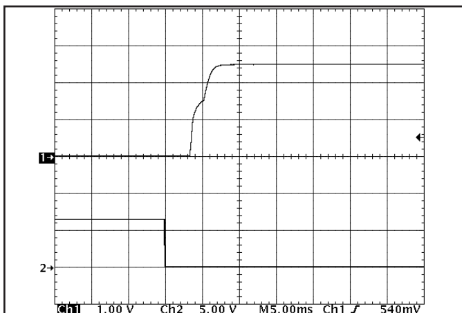
Figure 13: Turn-on transient at full rated load (resistive load) (5 ms/div). Input voltage pre-applied. Ch 1: Vout (1V/div). Ch 2: ON/OFF input (5V/div)
