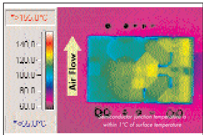
Figure 6: Thermal plot of converter at 51 amp load current with 55°C air flowing at the rate of 200 LFM. Air is flowing across the converter from pin 3 to pin 1 (nominal input voltage and 2 output pins).
