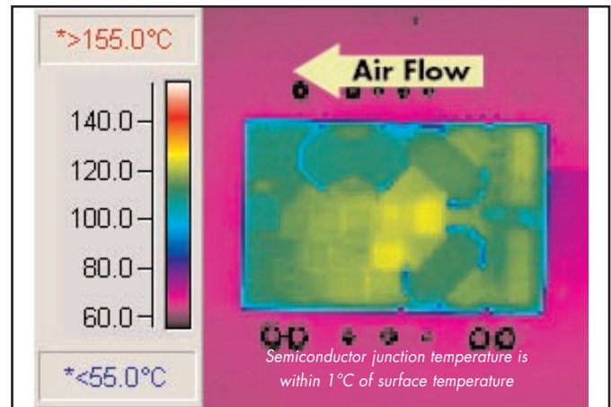
Figure 8: Thermal plot of converter at 49 amp load current with 55°C air flowing at the rate of 200 LFM. Air is flowing lengthwise from output to input (nominal input voltage and 2 output pins).
