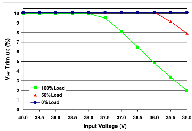
Figure 28: Achievable trim-up percentage vs. input voltage at output loads of 0%, 50% and full load (4 output pin unit).
