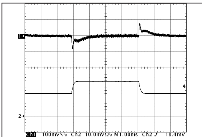
Figure 15: Output voltage response to step-change in load current (50%-75%-50% of I_{out(max)} ; dI/dt = 0.1A/\mu s ). Load cap: 10 \mu F , 100 m \Omega ESR tantalum cap and 1 \mu F ceramic cap. Ch 1: Vout (100mV/div), Ch 2: Iout (20A/div).
