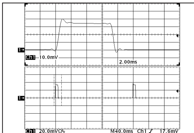
Figure 22: Load current (20 A/div) as a function of time when the converter attempts to turn on into a 1 m\Omega short circuit. Top trace (2 ms/div) is an expansion of the on-time portion of the bottom trace.
