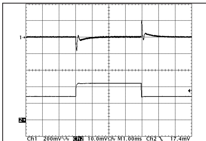
Figure 16: Output voltage response to step-change in load current (50%-75%-50% of I_{out(max)} ; dI/dt = 1A/\mu s ). Load cap: 470 \mu F , 30 m \Omega ESR tantalum cap and 1 \mu F ceramic cap. Ch 1: Vout (200mV/div), Ch 2: Iout (20A/div).
