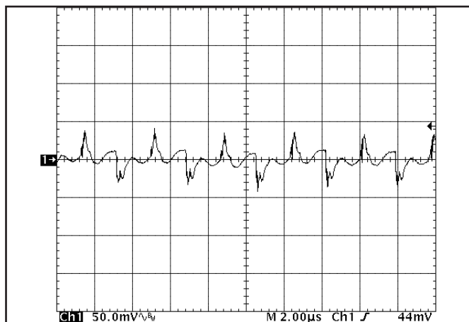
Figure 20: Output voltage ripple at nominal input voltage and rated load current (50 mV/div). Load capacitance: 1 \mu F ceramic capacitor and 10 \mu F tantalum capacitor. Bandwidth: 500 MHz. See Figure 17.
