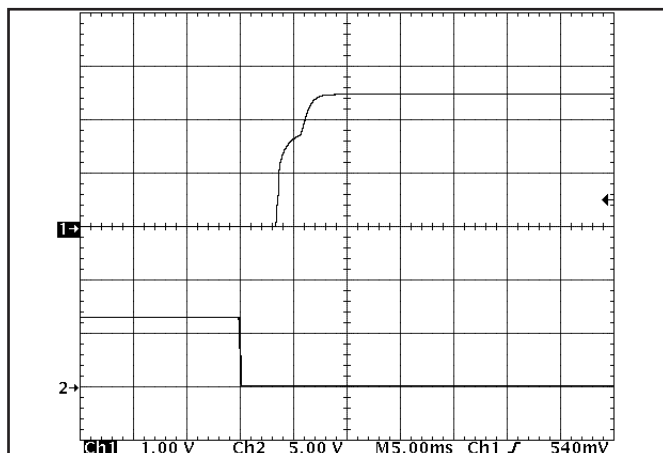
Figure 14: Turn-on transient at zero load current (5 ms/div). Ch 1: Vout (1V/div). Ch 2: ON/OFF input (5V/div).
