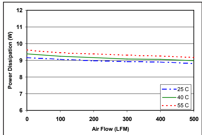
Figure 4: Power dissipation at nominal output voltage and 60% rated power vs. airflow rate for ambient air temperatures of 25°C, 40°C, and 55°C (nominal input voltage and 2 output pins).
