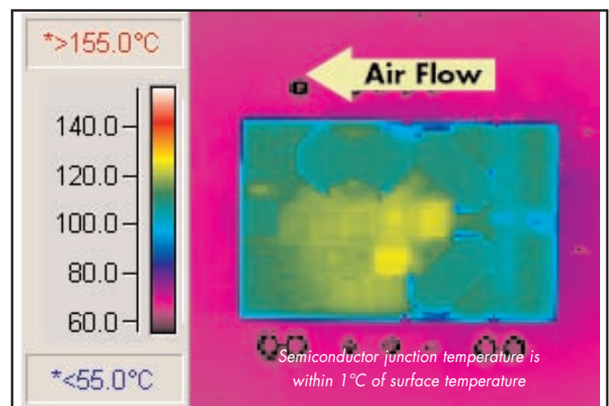
Figure 12: Thermal plot of converter at 53 amp load current with 55°C air flowing at the rate of 200 LFM. Air is flowing lengthwise from output to input (nominal input voltage and 4 output pins).
