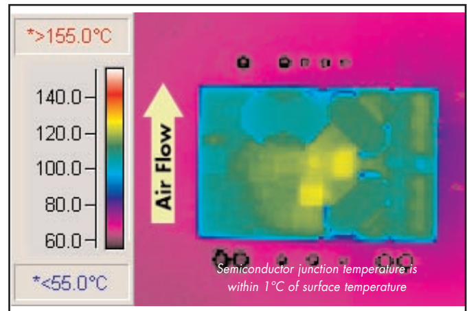
Figure 10: Thermal plot of converter at 55 amp load current with 55°C air flowing at the rate of 200 LFM. Air is flowing across the converter from pin 3 to pin 1 (nominal input voltage and 4 output pins).
