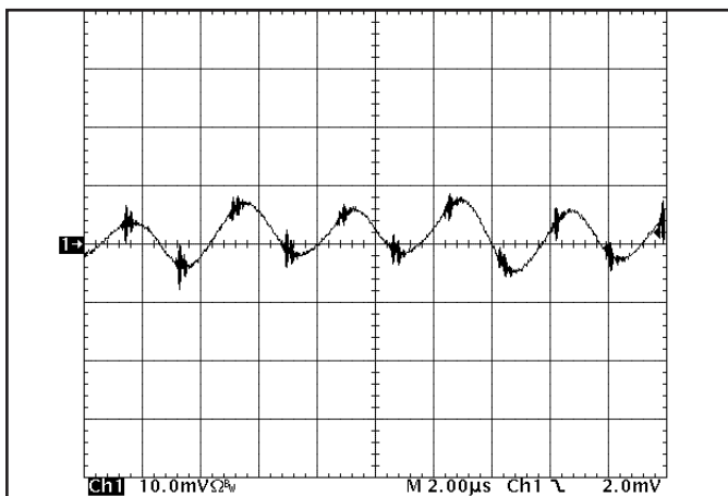
Figure 19: Input reflected ripple current, i_s , through a 10 \mu H source inductor at nominal input voltage and rated load current (5 mA/div). See Figure 17.
