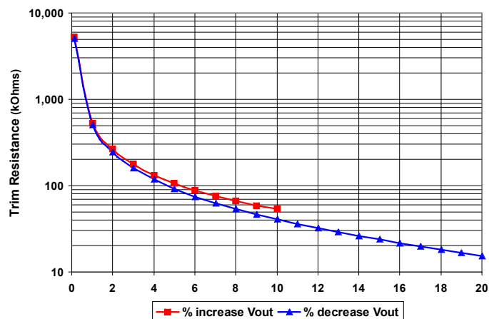
Figure C: Trim Graph for 2.5Vout module
