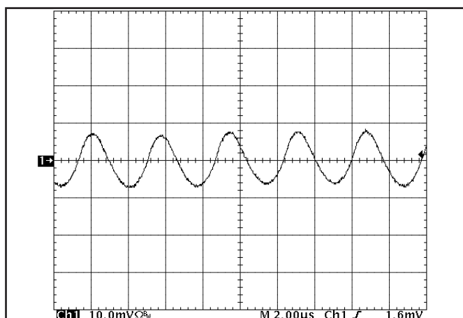
Figure 18: Input Terminal Ripple Current, i_C , at full rated output current and nominal input voltage with 10 \mu H source impedance and 47 \mu F electrolytic capacitor (200 mA/div). See Figure 17.
