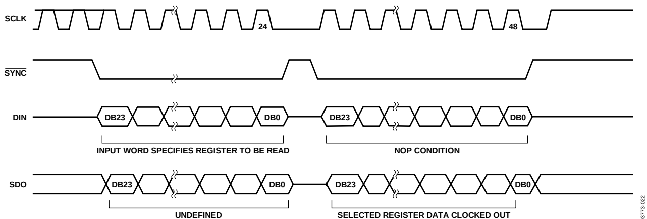
Figure 32. Readback Operation
