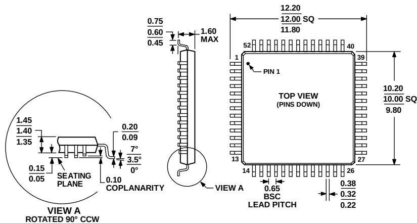
Figure 53. 52-Lead Low Profile Quad Flat Package [LQFP] (ST-52)
