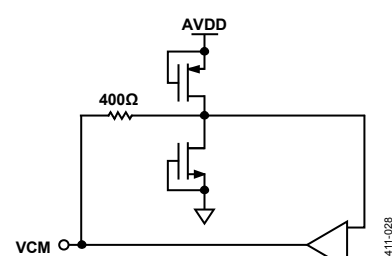
Figure 28. Equivalent VCM Circuit
