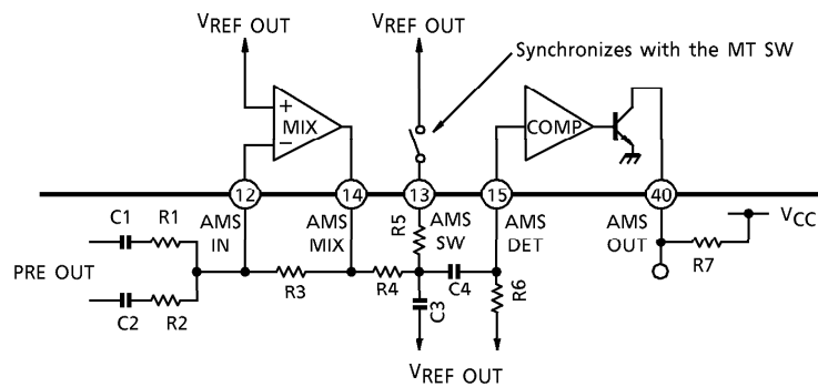
Fig.2 AMS system
