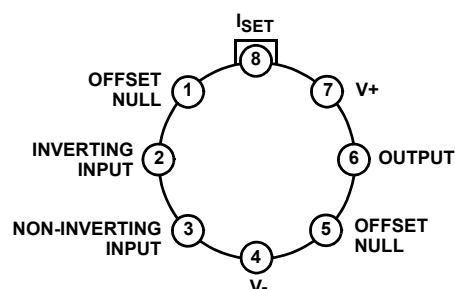
HS2-3530ARH, HS2-3530AEH (CAN), MACY1-X8 TOP VIEW
