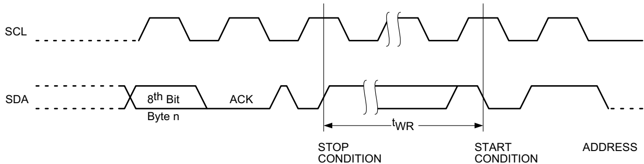
Figure 8. Write Cycle Timing
