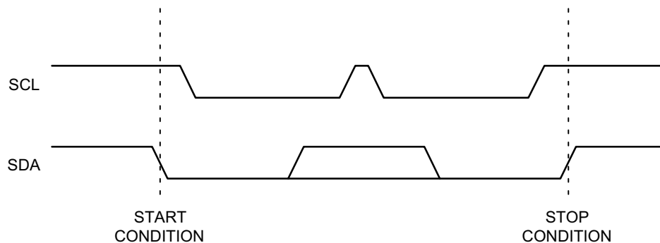
Figure 3. START/STOP Conditions
