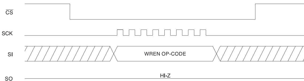
Figure 4-2. WREN Timing
