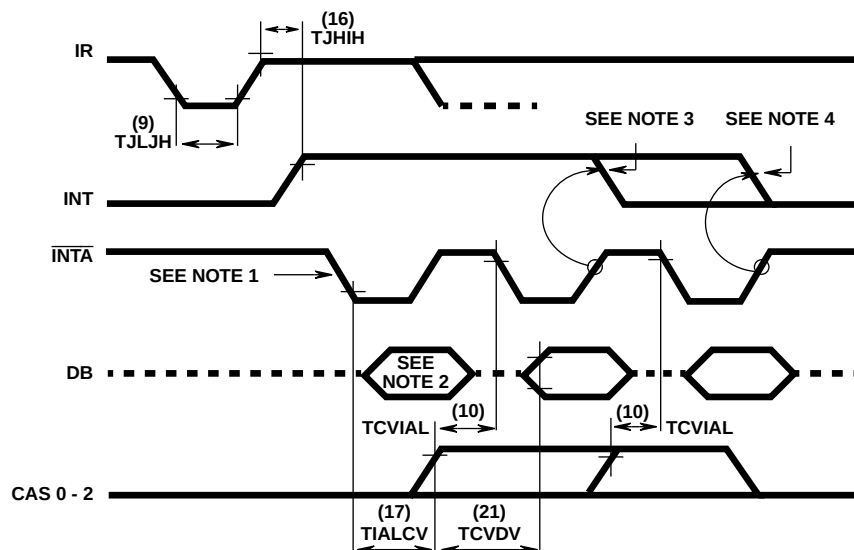
FIGURE 14. OTHER TIMING
