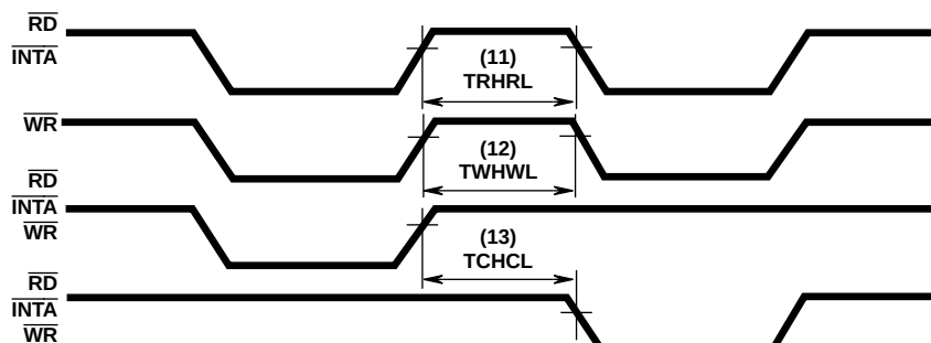
FIGURE 14. OTHER TIMING
