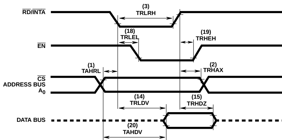
FIGURE 13. READ/INTA
