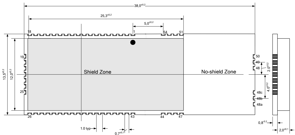
ZDM-A1281-PN/PN0 Mechanical Drawing
