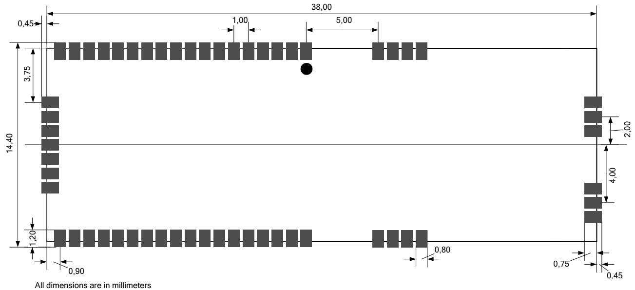
ZDM-A1281-PN/PN0 PCB Recommended Layout, Top View
