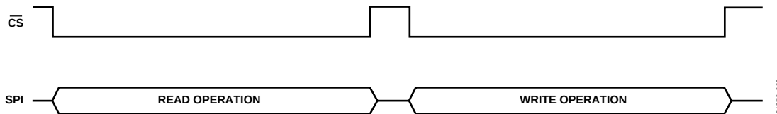
Figure 63. SPI—Correct Use of \overline{CS} During SPI Communication
