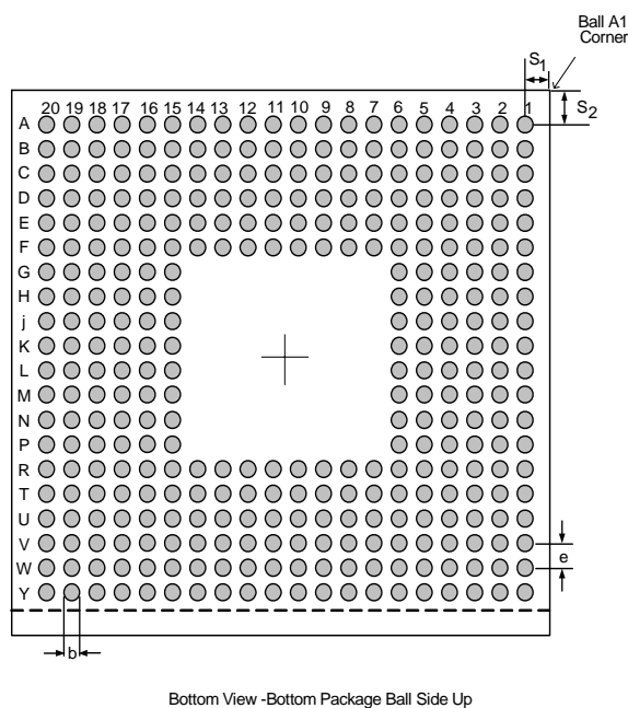
Figure 3-3. 14 x 14 mm Intel® PXA271 Processor Package, Bottom View
