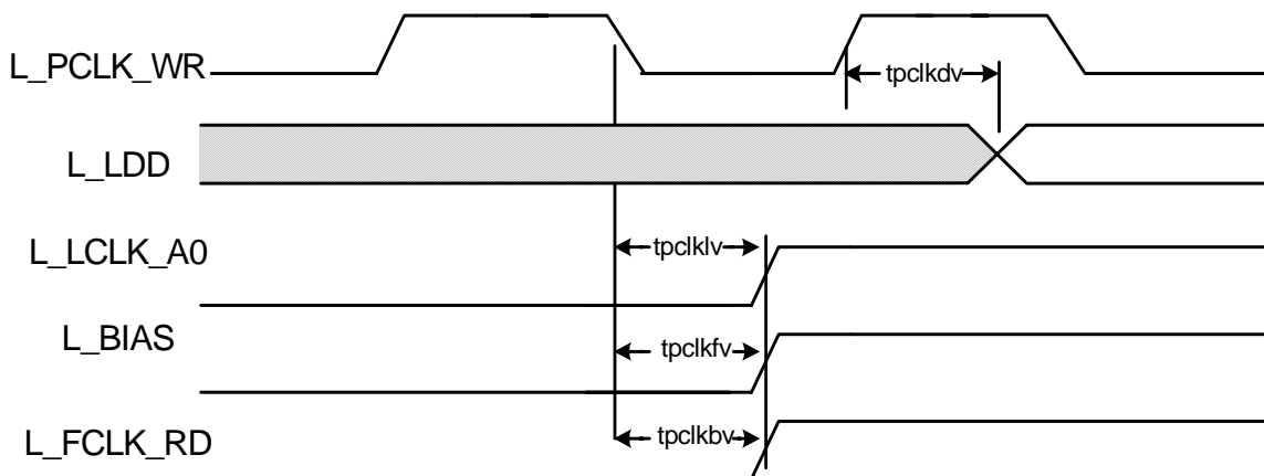
Figure 6-28. LCD Timing Definitions
