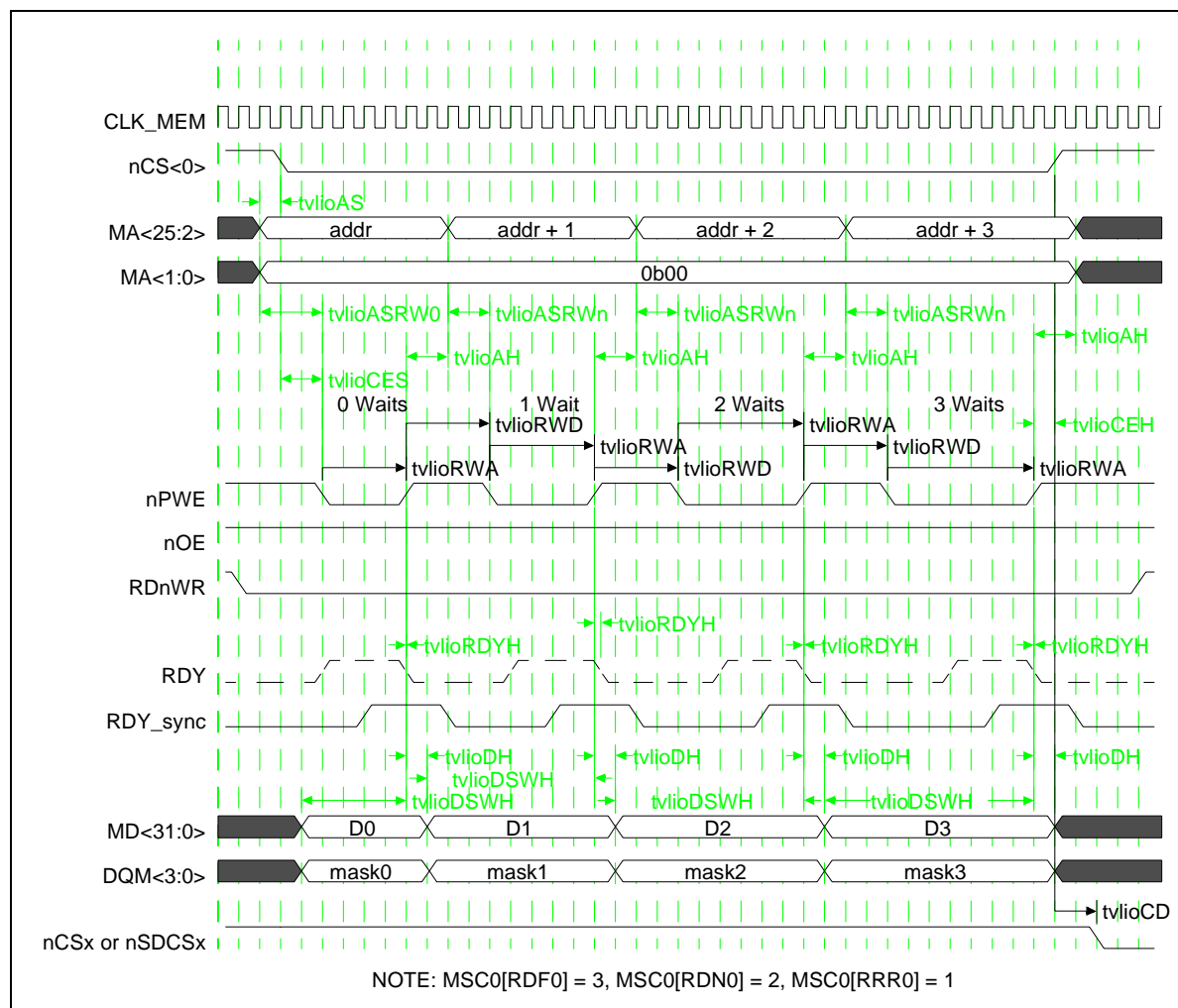
Figure 6-25. 32-Bit VLIO Write Timing
