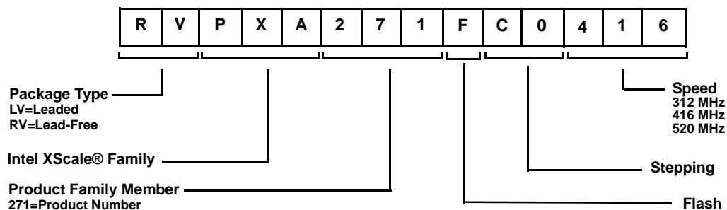
Figure 3-9. Intel® PXA27x Product Information Decoder
