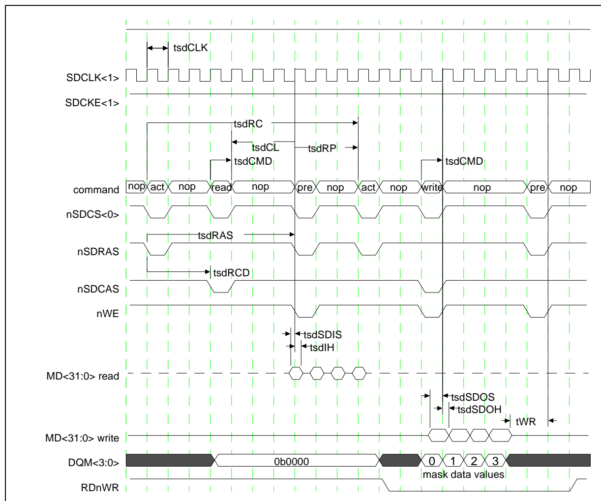
Figure 6-7. SDRAM Timing
