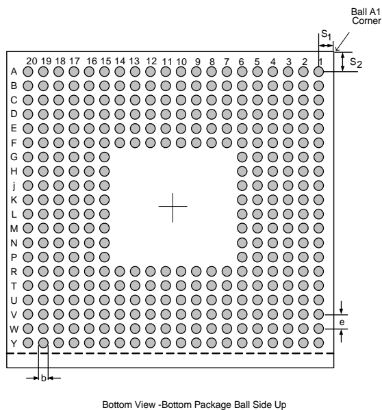
Figure 3-6. 14 x 14 mm Intel® PXA272 Processor Package, Bottom View
