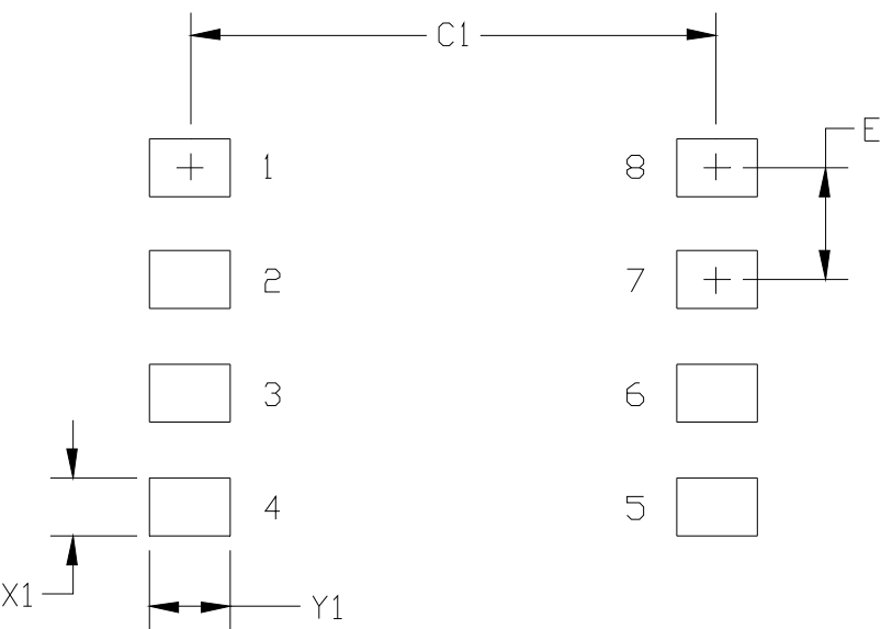
Figure 28. LGA8 Land Pattern
