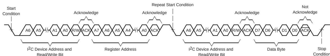
Figure 2–16. Single-Byte Read
