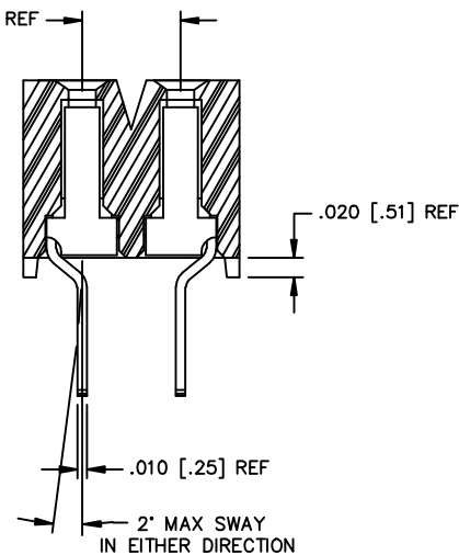
SECT. "A-A"
