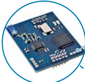
Fig. 1a - 2.4 GHz Wireless Sensor Module ; incl. TI MCU MSP430F2274 and radio CC2500. Auxiliary I 2 C digital inputs and programming interfaces on-board.
