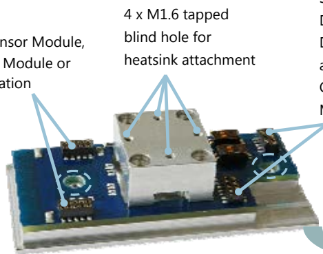
Fig. 5 - TE-Power Base assembly with heatsink adaptor and routing PCB. Module interfaces and TEG polarity-inverting DIP switches.
