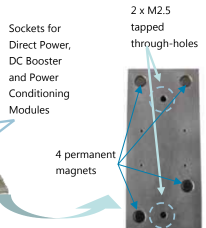
Fig. 6 - Bottom of TE-Power Base assembly with permanent magnets and tapped mounting holes for easy attachment to surfaces and adaptors.
