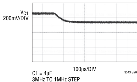
PLL Operation
