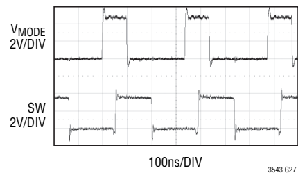
PLL Operation at 3MHz
