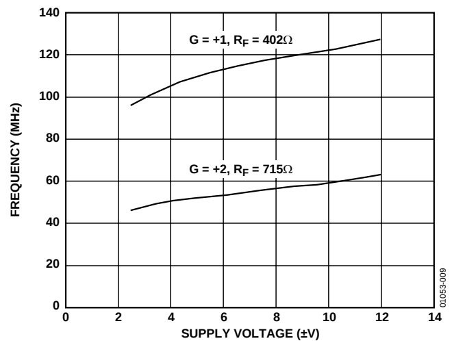
Figure 9. Bandwidth vs. Supply, R_L = 500\text{ }\Omega , V_{IN} = 200\text{ mV p-p}
