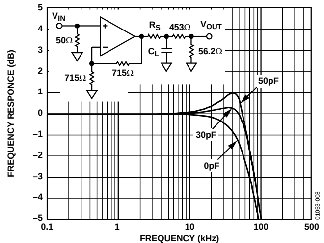
Figure 8. Frequency Response vs. Capacitive Load; C_L = 0\text{ pF} and 50\text{ pF} ; R_S = 0\text{ }\Omega
