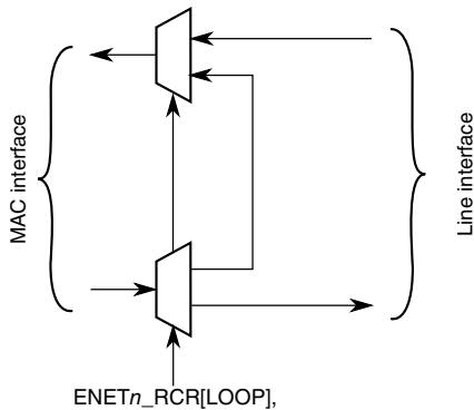
Figure 44-63. Loopback Options
