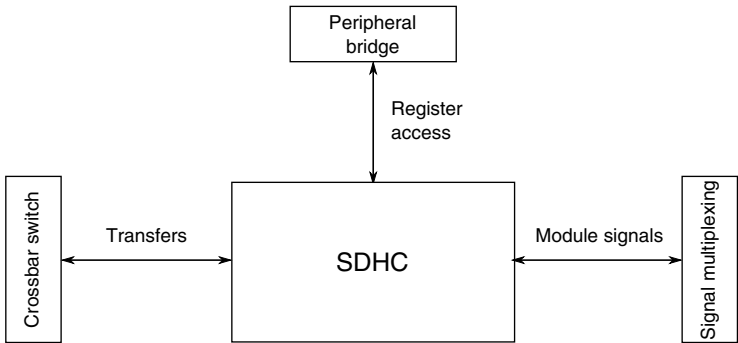
Figure 3-63. SDHC configuration
