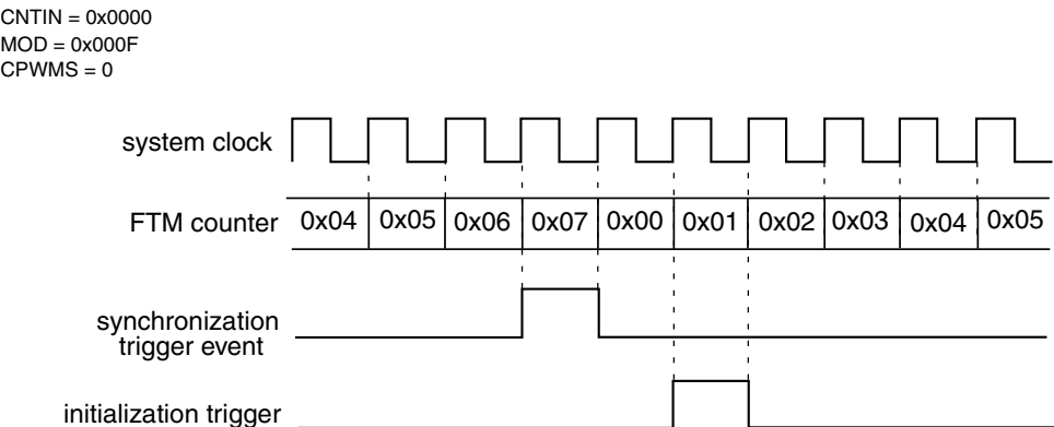
Figure 39-241. Initialization Trigger Is Generated When There Is the FTM Counter Synchronization
