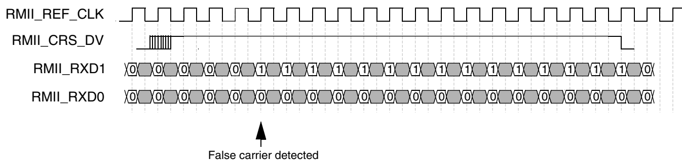
Figure 44-70. RMI receive operation with false carrier
