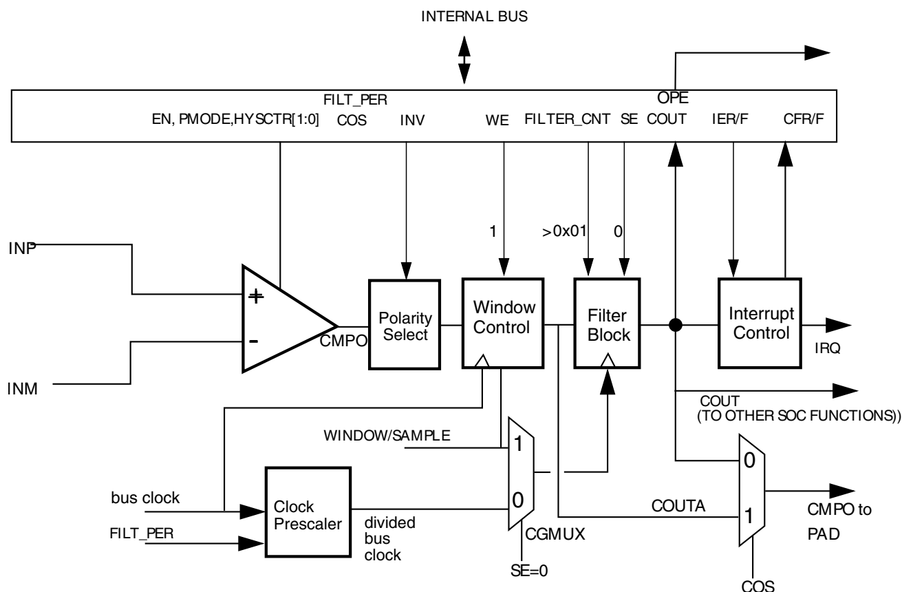
Figure 35-35. Windowed/Filtered Mode
