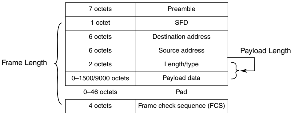
Figure 44-52. MAC Frame Format Overview
