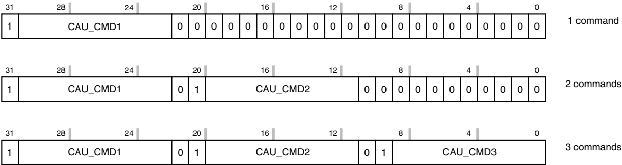
Figure 32-16. Direct loads
