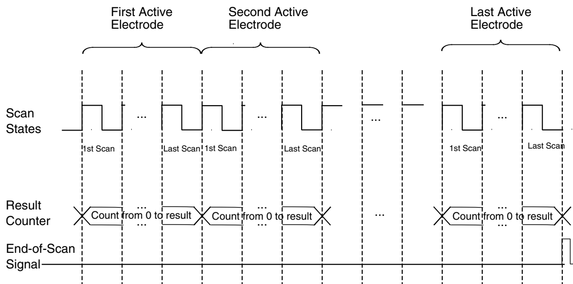
Figure 55-71. Scan sequence
