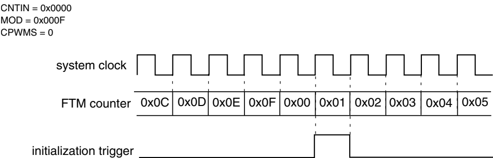
Figure 39-239. Initialization Trigger Is Generated When the FTM Counting Achieves the CNTIN Register Value
