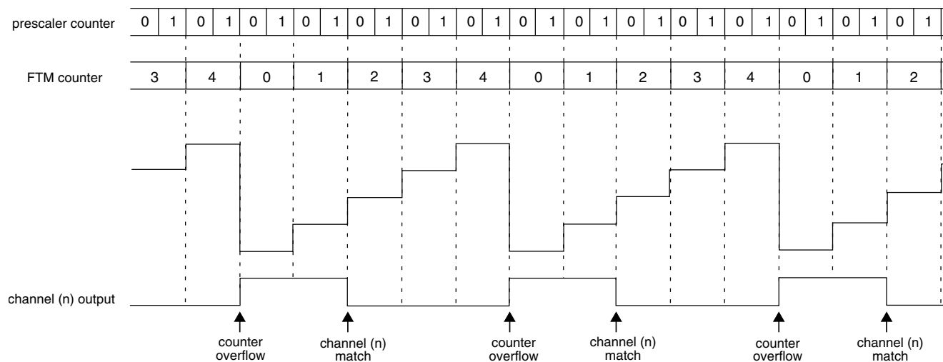
Figure 39-166. Notation Used
