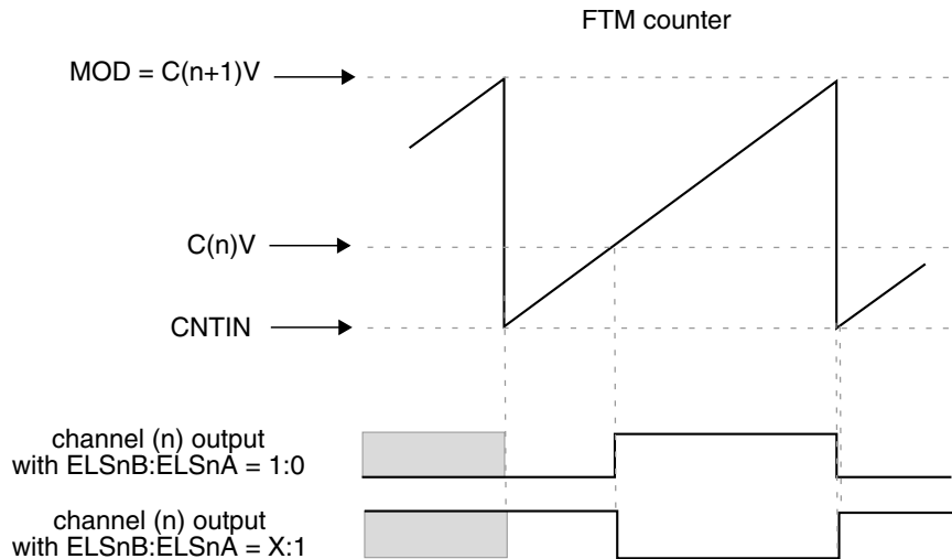
Figure 39-189. Channel (n) Output If (CNTIN < C(n)V < MOD) and (C(n+1)V = MOD)
