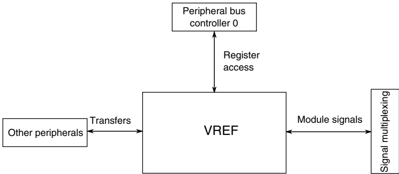
Figure 3-42. VREF configuration
