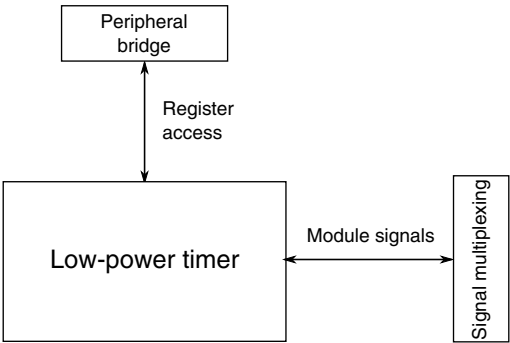
Figure 3-48. LPT configuration
