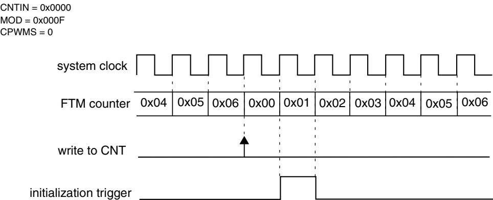
Figure 39-240. Initialization Trigger Is Generated When There Is a Write to CNT Register
