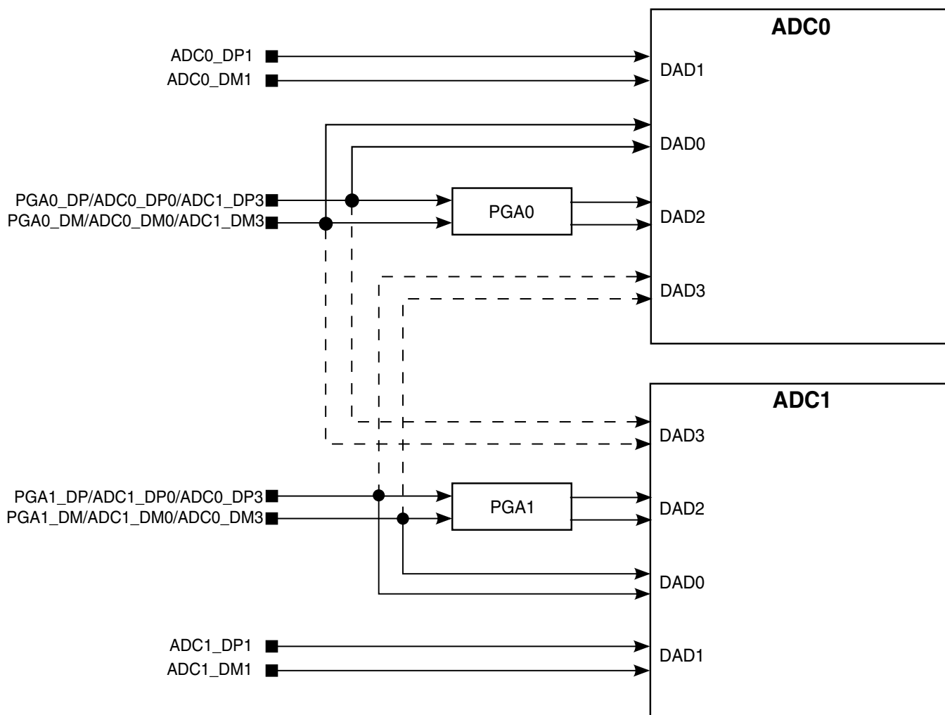
Figure 3-39. PGA Integration
