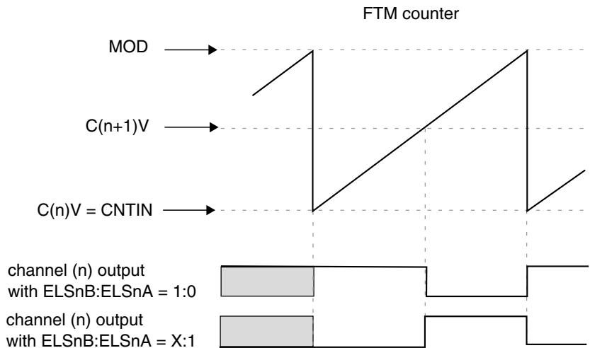
Figure 39-190. Channel (n) Output If (C(n)V = CNTIN) and (CNTIN < C(n+1)V < MOD)
