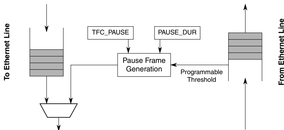
Figure 44-58. Pause Frame Generation Overview
