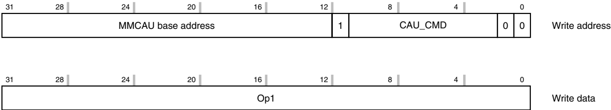
Figure 32-17. Indirect loads
