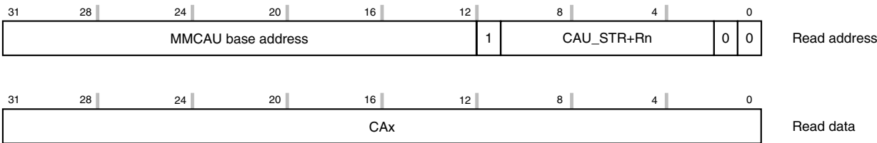
Figure 32-18. Indirect store
