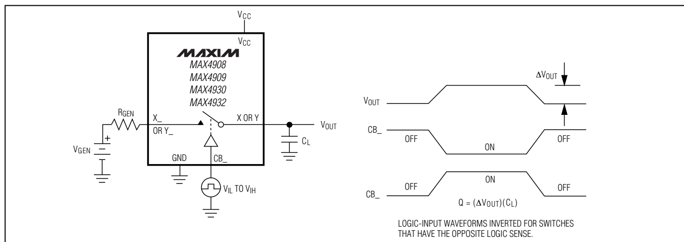
Figure 4. Charge Injection
