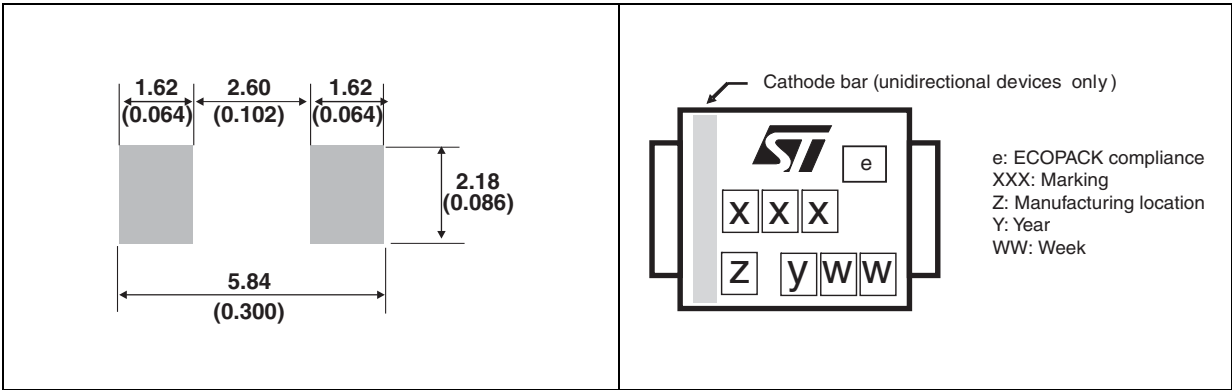
Figure 13. SMB footprint dimensions in mm (inches)
