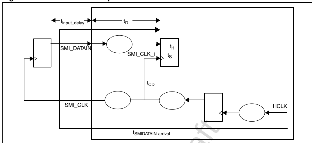
Figure 37. SMIDATAIN data path
