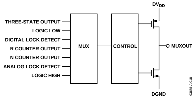
Figure 20. MUXOUT Schematic
