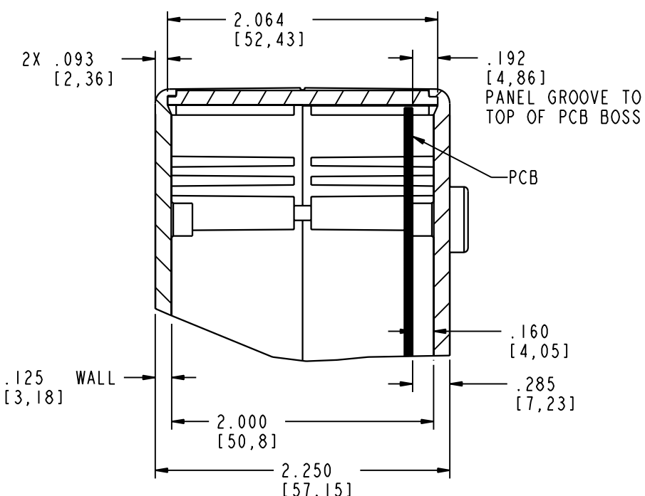
SECTION C-C
