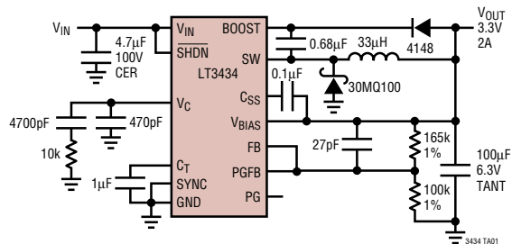
14V to 3.3V Step-Down Converter with 100μA No Load Quiescent Current
