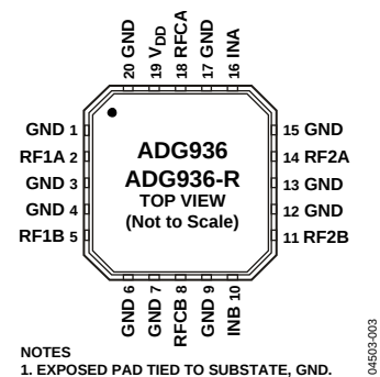
Figure 6. 20-Lead 4 mm x 4 mm LFCSP (CP-20-1)
