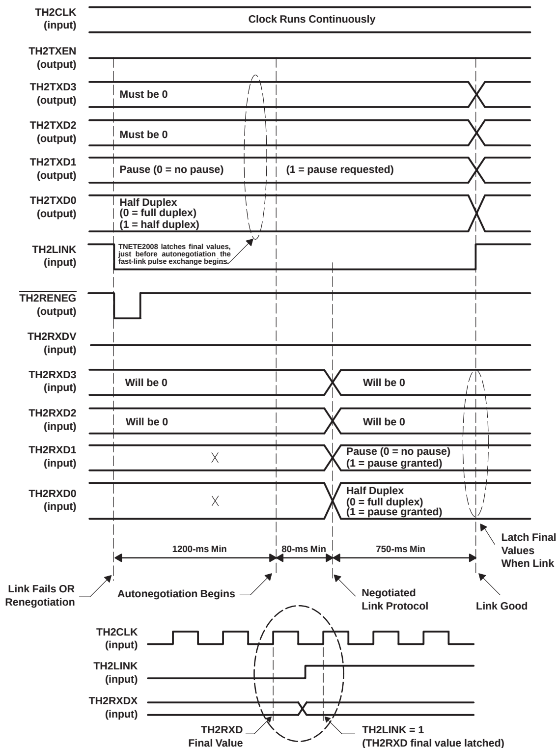
Figure 6. Connecting to TNETE2008 PHY
