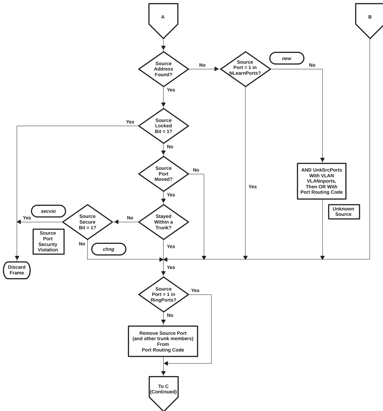
Figure 8. Frame-Routing Algorithm (Continued)
