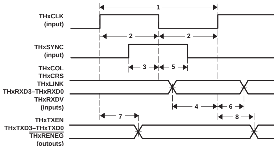
Figure 12. 10-Mbit/s Interface (Ports 00–07)
