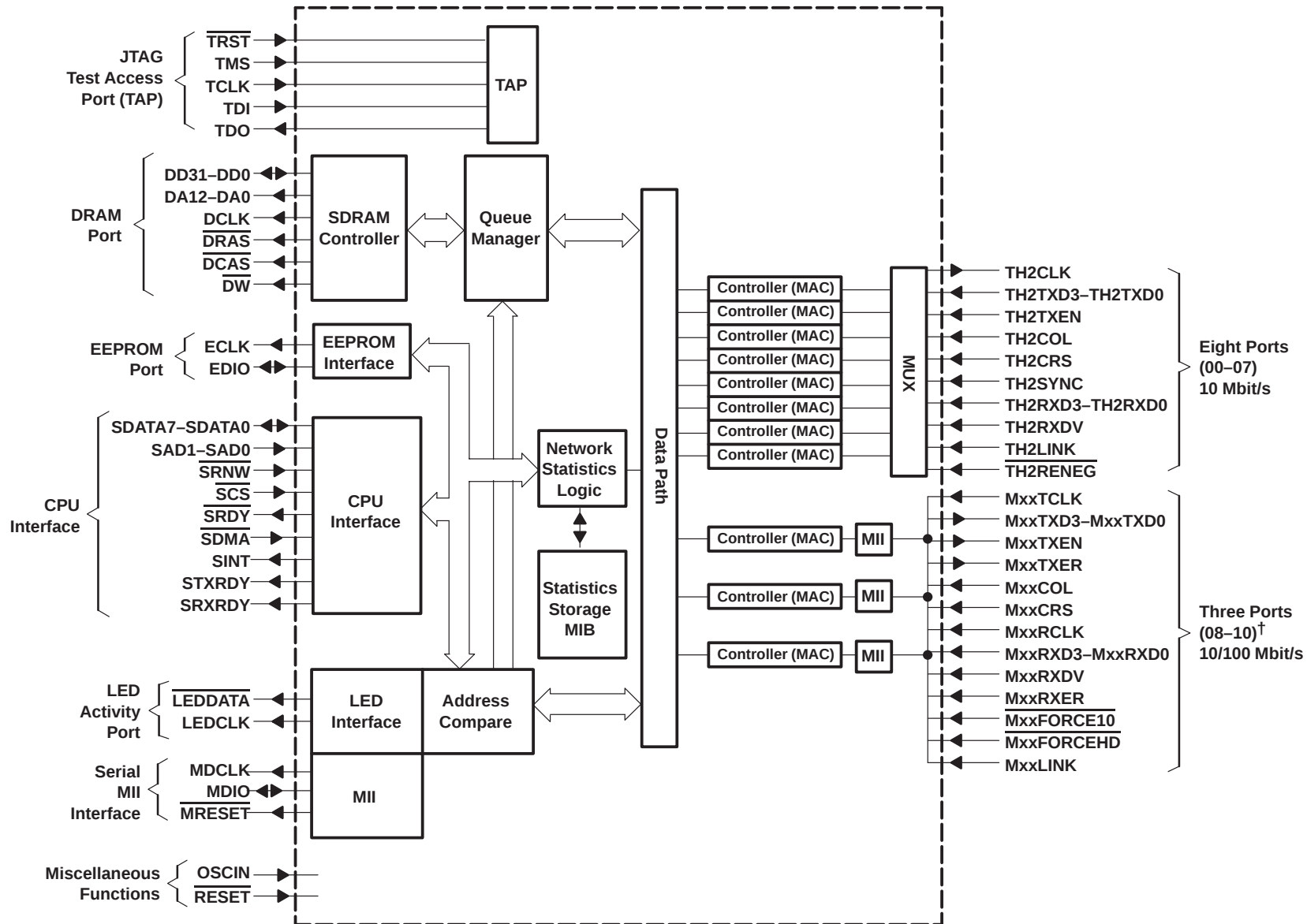
Figure 1. TNETX3110 Interface Block Diagram
