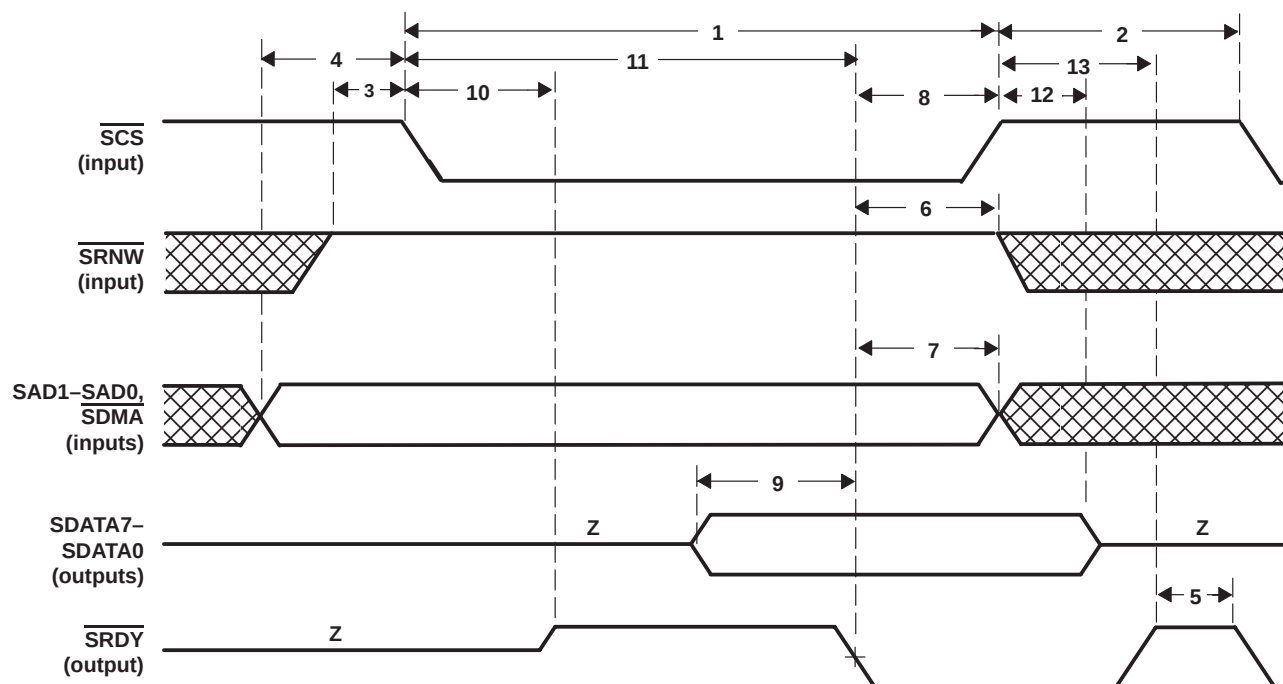
Figure 18. DIO/DMA Read Cycle
