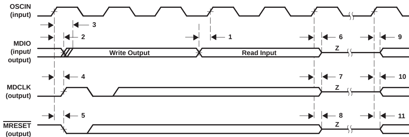
Figure 19. Serial MII Management Read/Write Cycle
