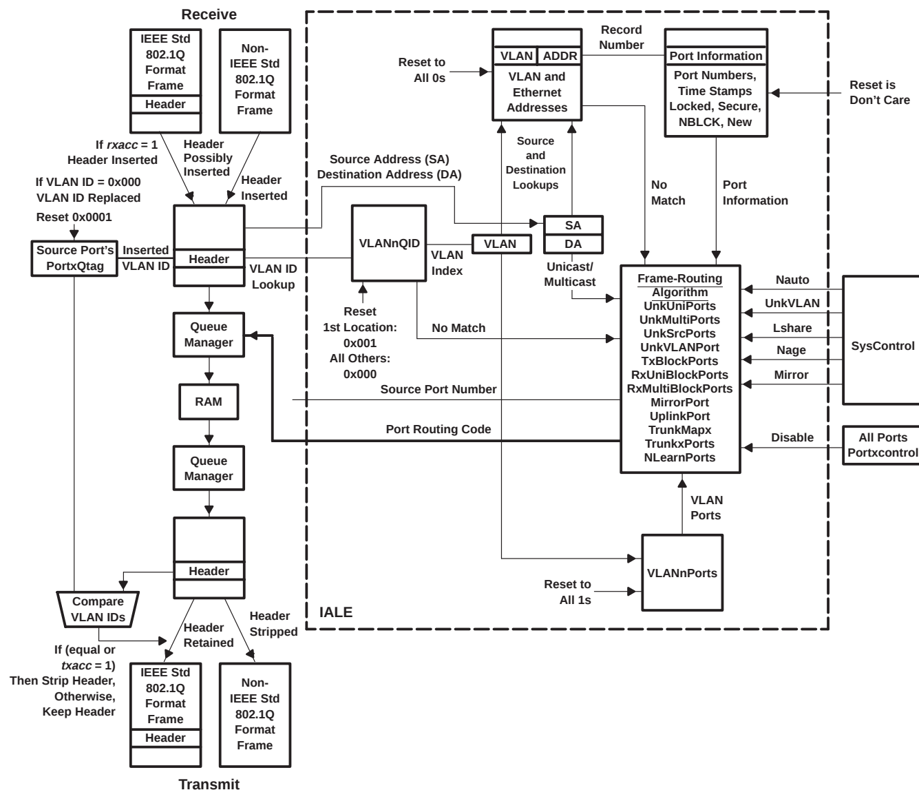
Figure 7. VLAN Overview
