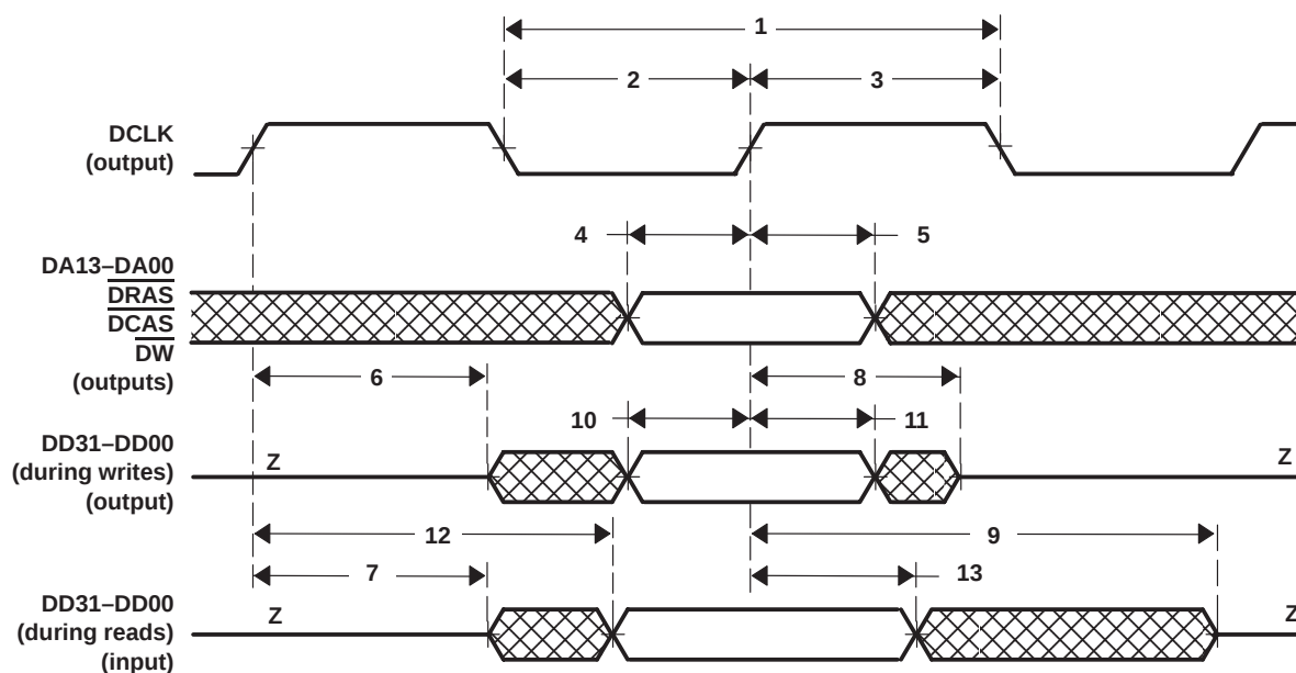
Figure 16. SDRAM Subcycle
