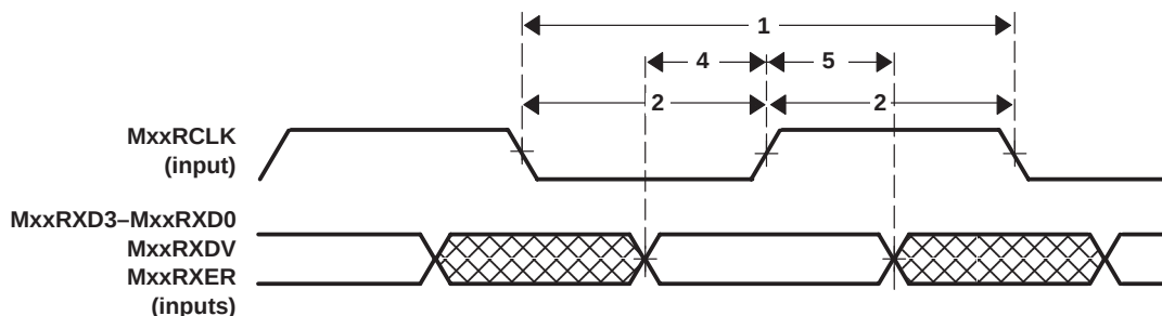
Figure 13. 10-/100-Mbit/s Receive Ports
