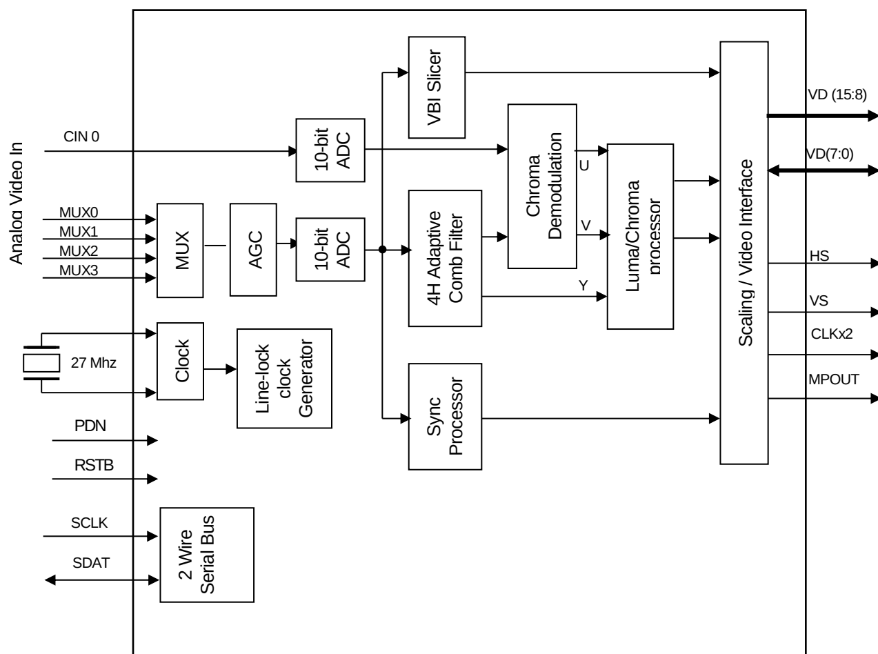
FIGURE 1. TW9910 BLOCK DIAGRAM
