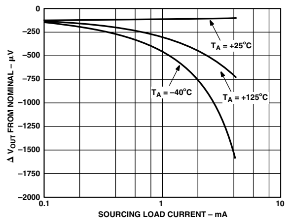
TPC 12. ADR291 \Delta V_{OUT} from Nominal vs. Load Current
