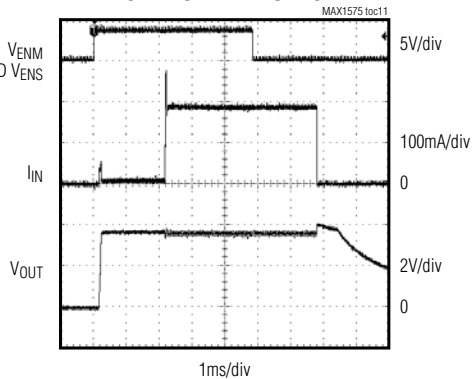
STARTUP WAVEFORMS
