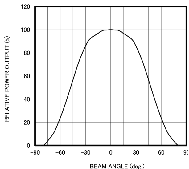
RADIATION PATTERN
