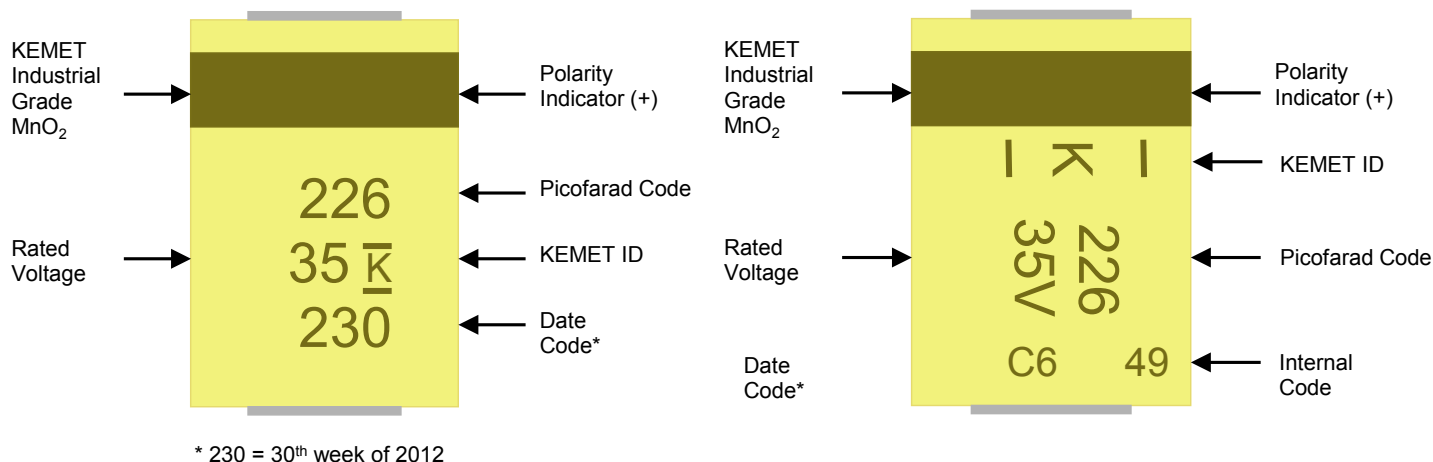
C, D, X Case Sizes
