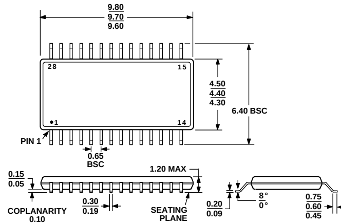
Figure 63. 28-Lead Thin Shrink Small Outline Package [TSSOP] (RU-28)
